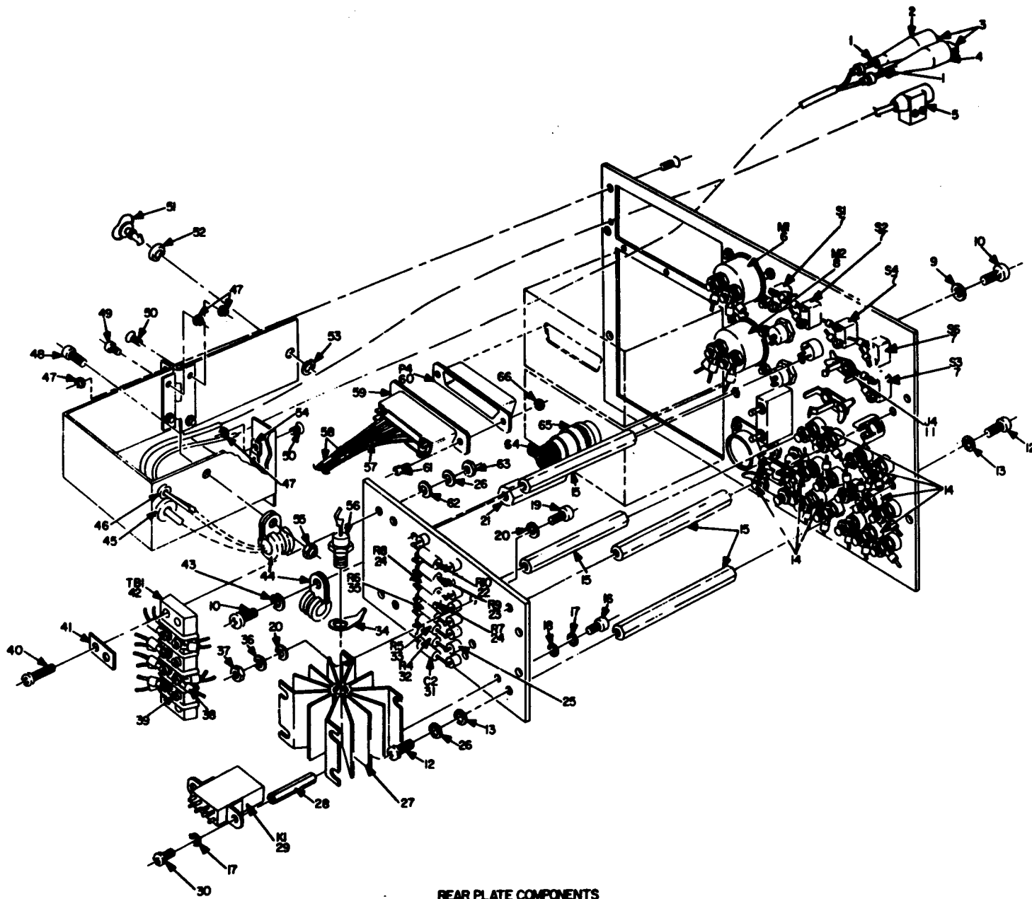
Figure 2. Test Panel SB-3716(P)/ARC (Modified) (Sheet 1 of 2).
